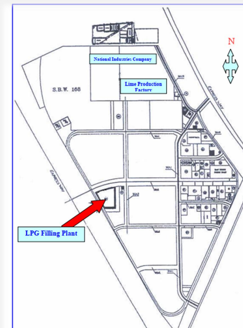
Fig. 1 The LPG Filling plant project area location within Shuaiba Industrial Area (SIA) western sector.
